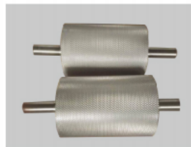
Beeswax foundation roller 3801007-450mm x86mm 3801008-450mm x170mm
